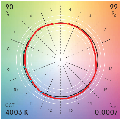
Figure 2 - Colour Vector Graphics for 4000K, 90CRI
