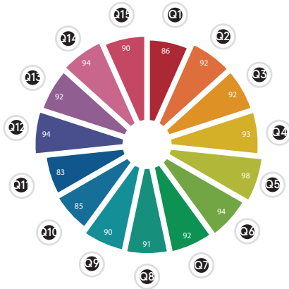
Figure 3 - Colour Quality Scale for 4000K, 90CRI
