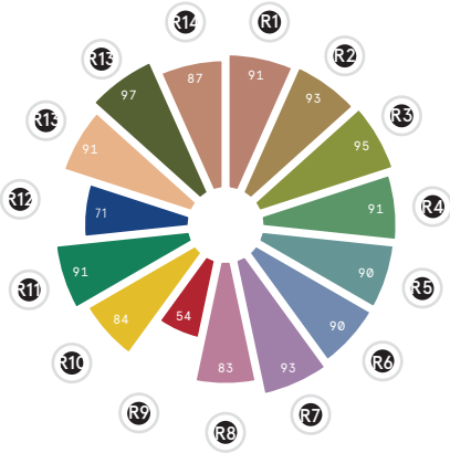
Figure 1 - Colour Rendering Index for 4000K, 90CRI
