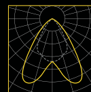
Batwing
